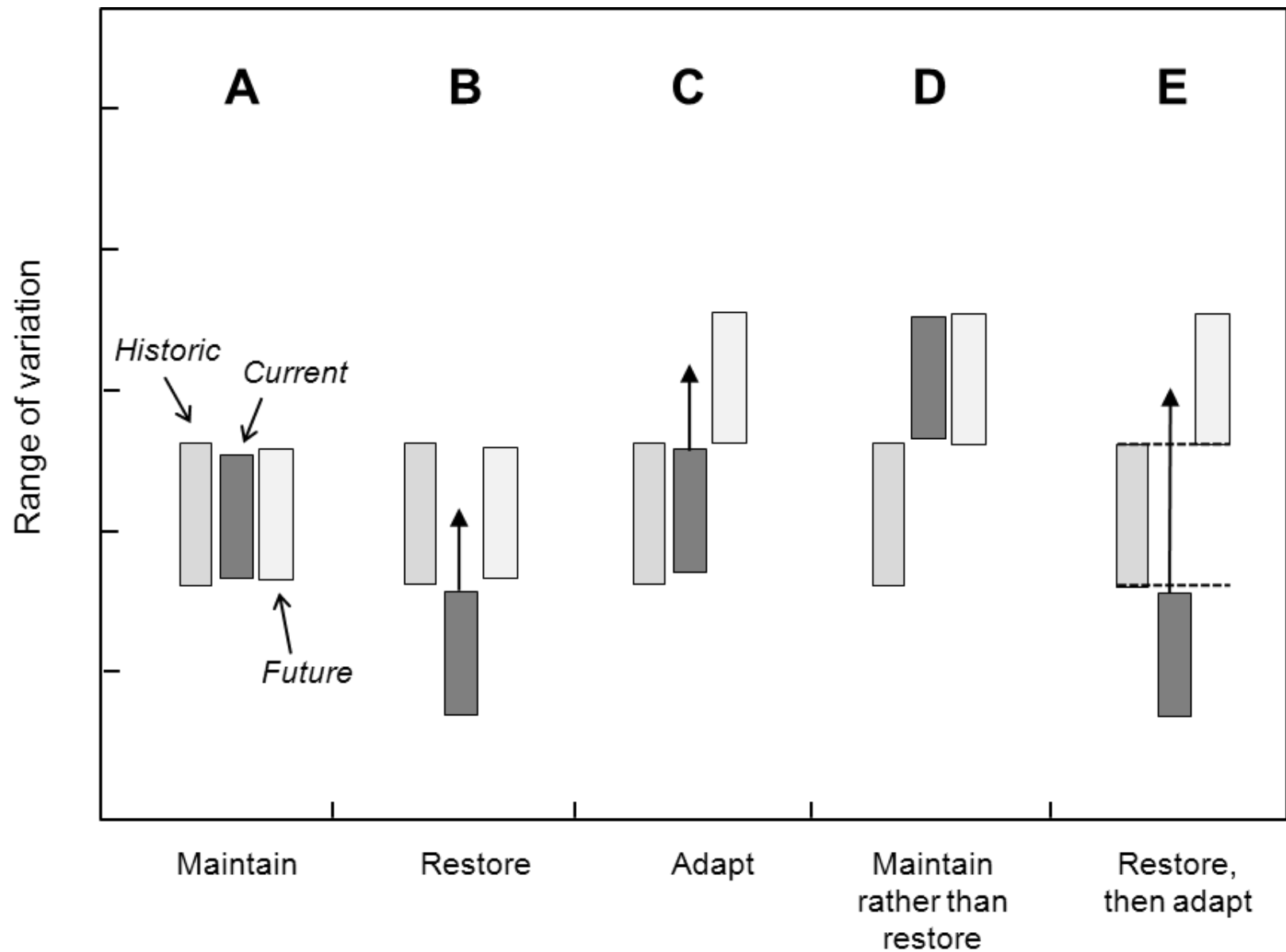
Fig. 4.2. Comparison of historic (medium gray), current (dark gray) and projected future (light gray) ranges of variation for a given ecological variable. From Safford et al. 2012.
